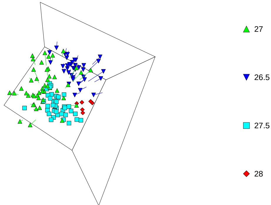
Figure 9.4.5. MDS of bycatch from the deepwater eastern king prawn fishery showing strong evidence (global R = 0.429 ) of latitudinal grouping. Legend in latitude (degrees south).
