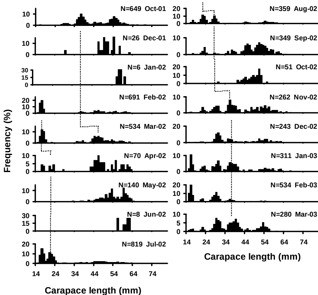
Figure 17.4.7. Monthly carapace length-frequency distributions for male Ibacus chacei . The dotted line outlines the suggested moult pattern for individuals recruiting to the fishery in February. Note: y-axis ranges vary.
