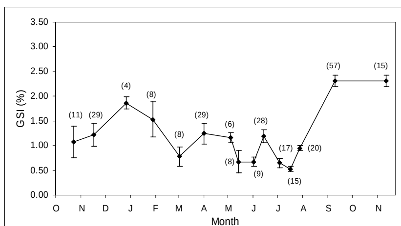
Figure 18.4.9. Gonadosomatic index for female N. theodorei between November 2001 and November 2002. Numbers in brackets indicate sample size
