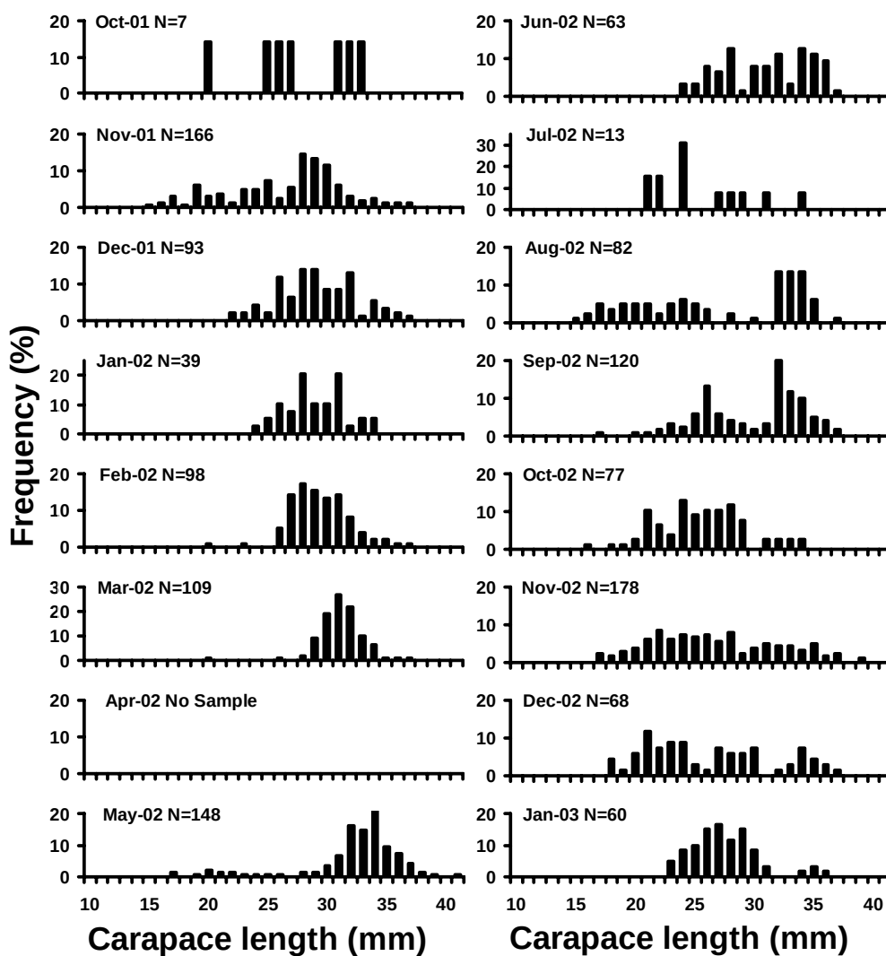
Figure 15.4.11. Monthly carapace length-frequency distributions of female Oratosquilla stephensoni (all data pooled). Note: y-axis ranges vary.
