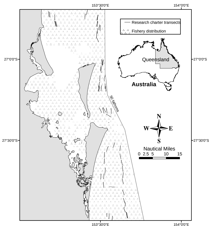
Figure 5.4.1. Location of the 60 two-nautical mile trawl sites in the shallow water eastern king prawn fishery that were sampled during the experimental research charter. Measures of prawn catches, bycatch and bycatch sub-samples were obtained from two nets (port and starboard) towed simultaneously at each location. Each “transect” is comprised of approximately 50 location data point readings taken directly from the vessel’s global positioning system at one-minute intervals while trawling and imported into a geographic information mapping program (ArcVIEW) for presentation.
