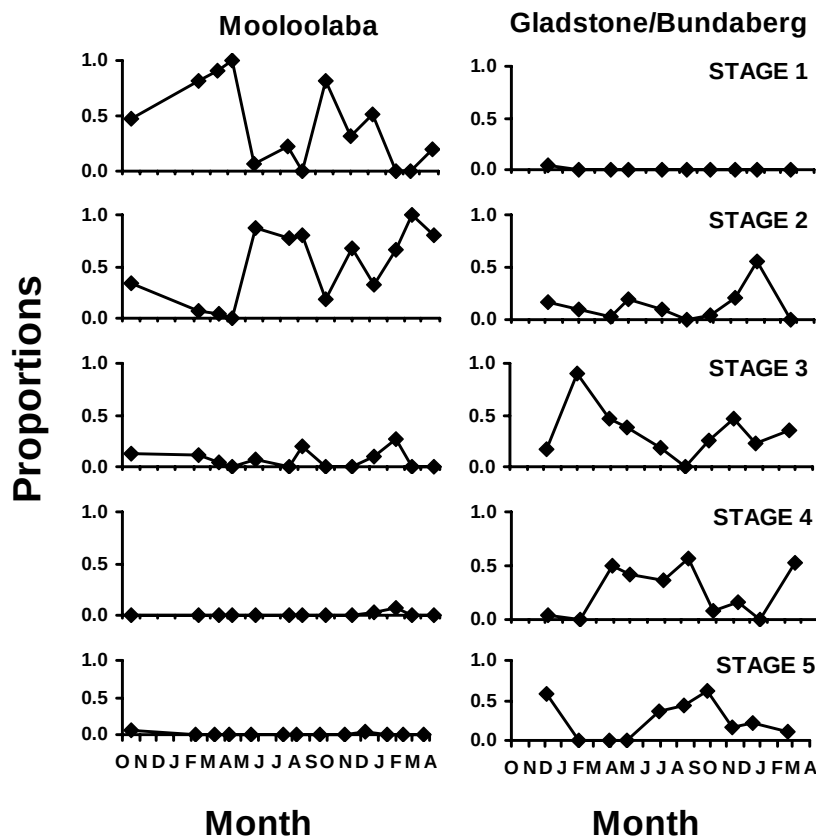
Figure 17.4.3. Seasonal changes in the proportions of adult female Ibacus chacei caught off Mooloolaba or Gladstone–Bundaberg in relation to ovarian maturation stages
