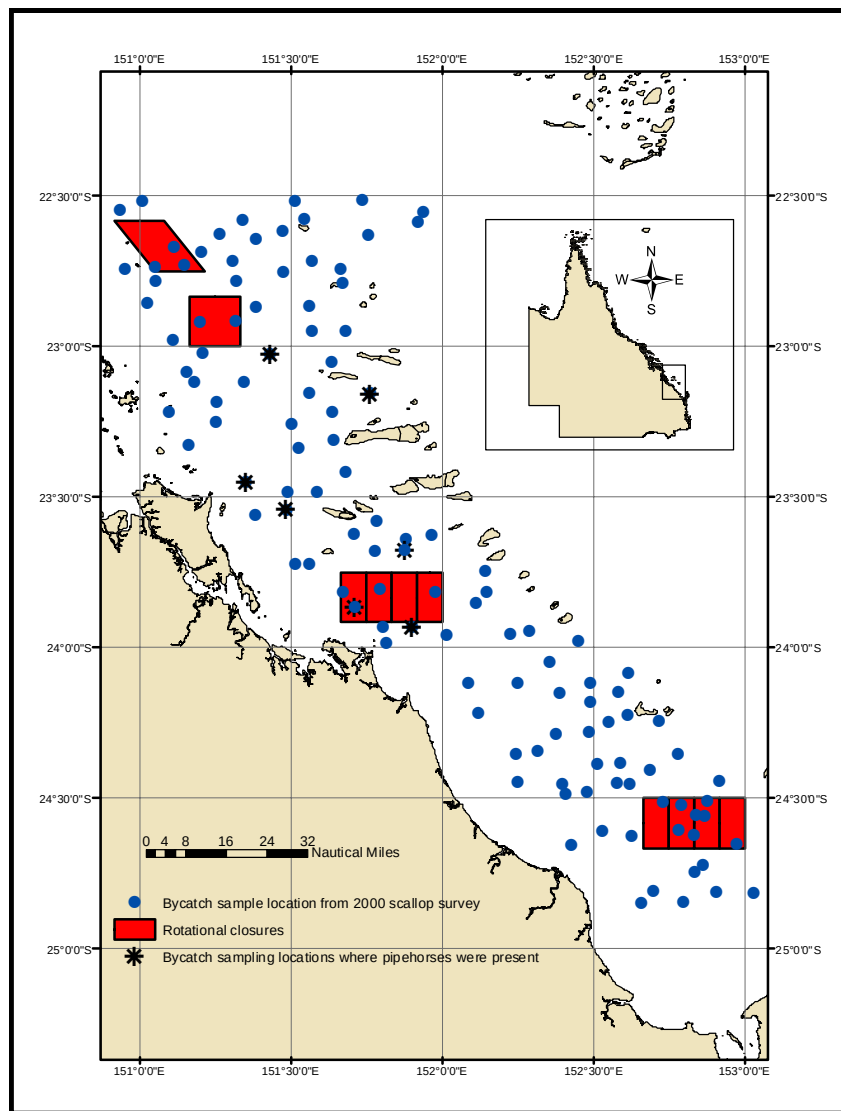
Figure 16.3.1. The location of 122 sites where bycatch was sampled during the 2000 Long Term Monitoring scallop fishery-independent survey. Pipehorses were present in trawls from seven of the 122 locations.
