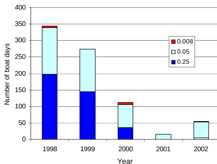
Figure 8.4.1. Number of boat-days in April and May each year on which fishing locations were reported at three levels of spatial precision (0.25: grid; 0.05: sub-grid; 0.008: lat-long) in Grid V33.
