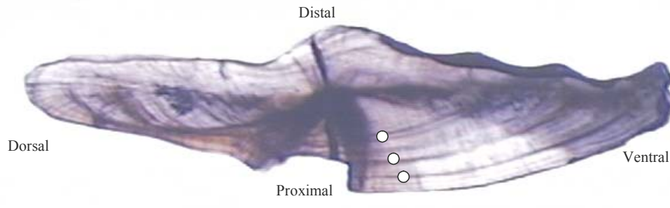
Figure 1. A transverse section of a N. theodorei otolith viewed with transmitted light. White circles indicate position of presumed annual increments. Scale bar =1mm
