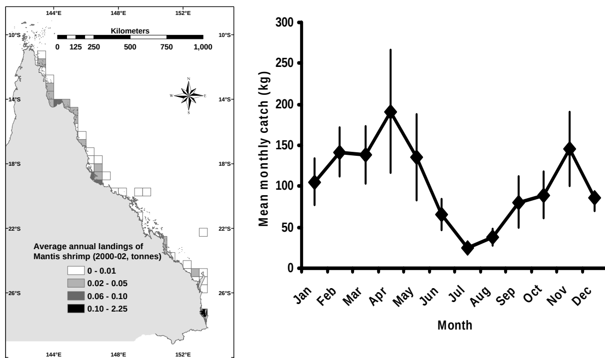
Figure 15.4.1. Spatial and temporal trends of reported mantis shrimp landings from the Queensland East Coast Trawl Fishery
