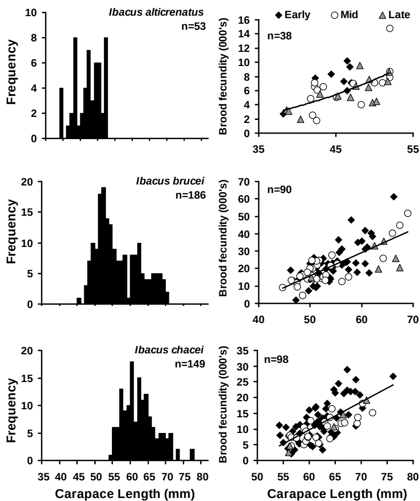
Figure 17.4.4. Size-frequency distributions of ovigerous females and scatterplot regressions of brood fecundity and carapace length for Ibacus alticrenatus , Ibacus brucei and Ibacus chacei . Note: y-axis ranges vary.
