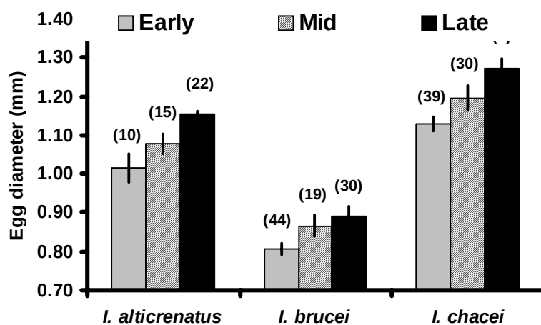
Figure 17.4.5. Comparisons of mean egg size ( \pm 95% CI) with egg development for Ibacus alticrenatus , Ibacus brucei and Ibacus chacei . Sample numbers in parentheses.
