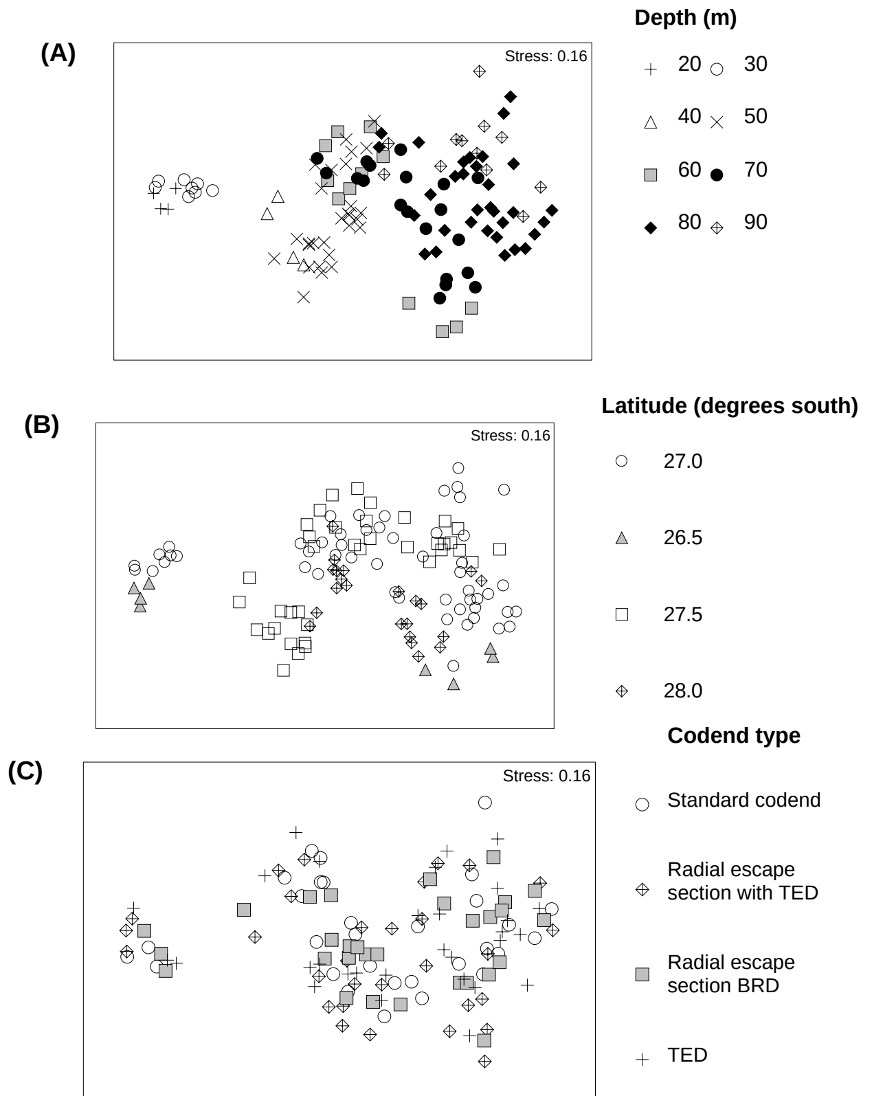
Figure 5.4.3. Two-dimensional MDS of bycatch sub-samples from an experimental research charter undertaken in the Queensland shallow water eastern king prawn trawl fishery. Catch rates were square-root transformed. The analyses used all 120 sub-samples and 118 species. Factors examined were (A) depth, (B) latitude and (C) codend type.
