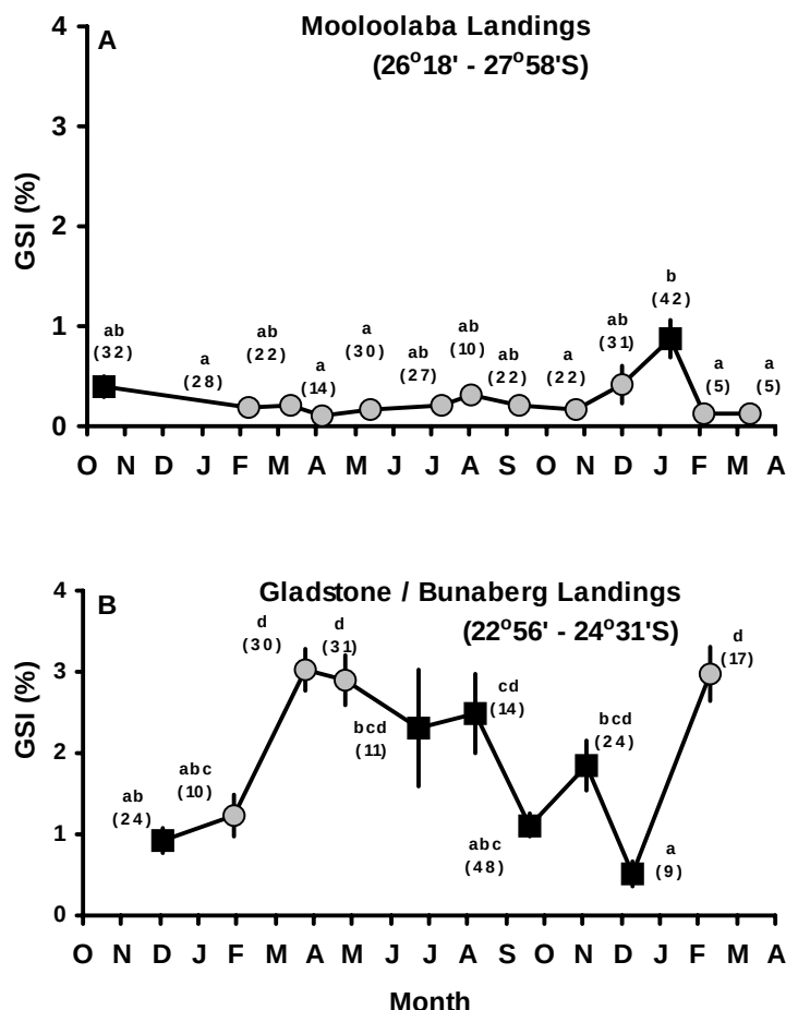
Figure 17.4.2. Seasonal changes in mean gonadosomatic index (GSI \pm S.E.) from adult female Ibacus chacei (> 54 mm CL) caught off (A) Mooloolaba or (B) Gladstone–Bundaberg from October 2001 to March 2003. ■ Indicates samples where ovigerous females were present. Values that are significantly different have different superscripts ( P < 0.05 ). Sample numbers given in parentheses.
