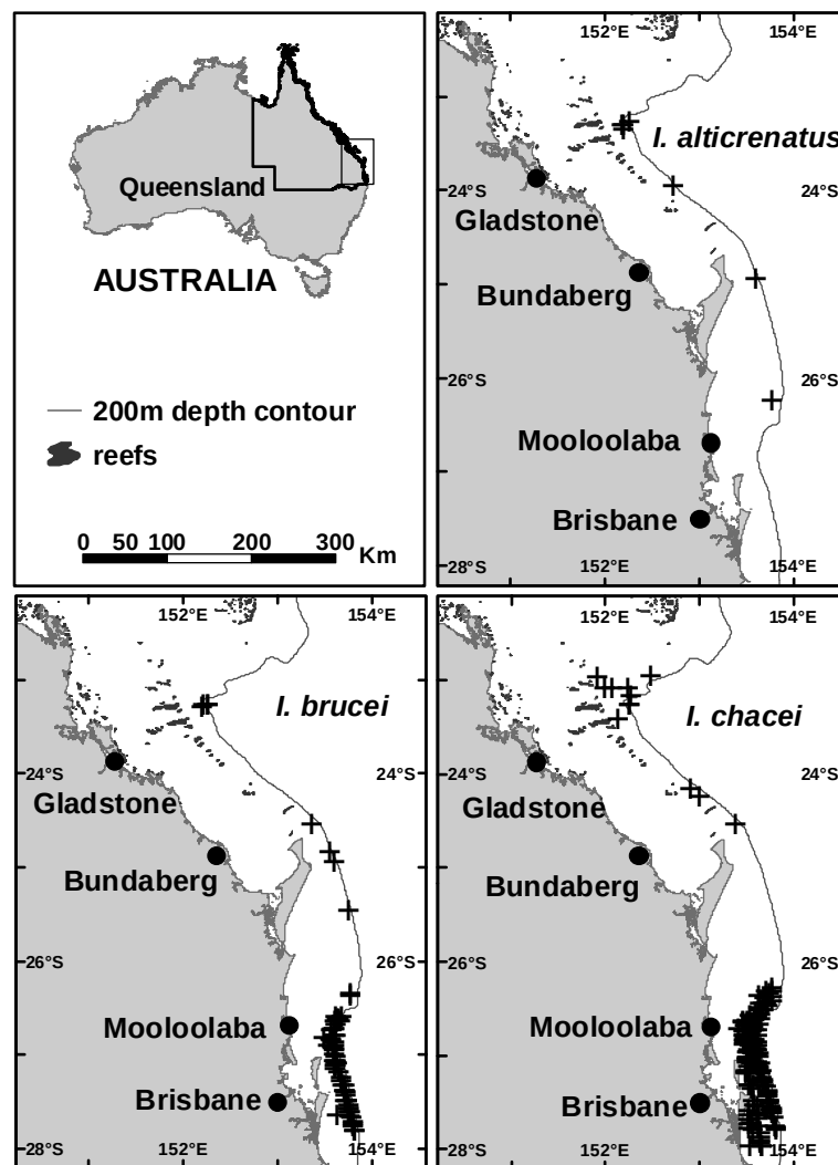
Figure 17.3.1. Sample location sites. Crosses indicate exact locations where samples were obtained.
